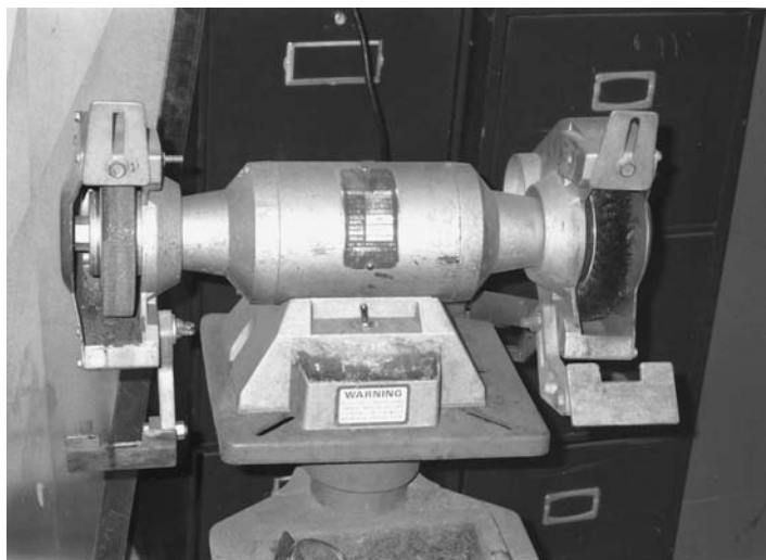
FIGURE 25.1 Example of a very unsafe abrasive wheel.
