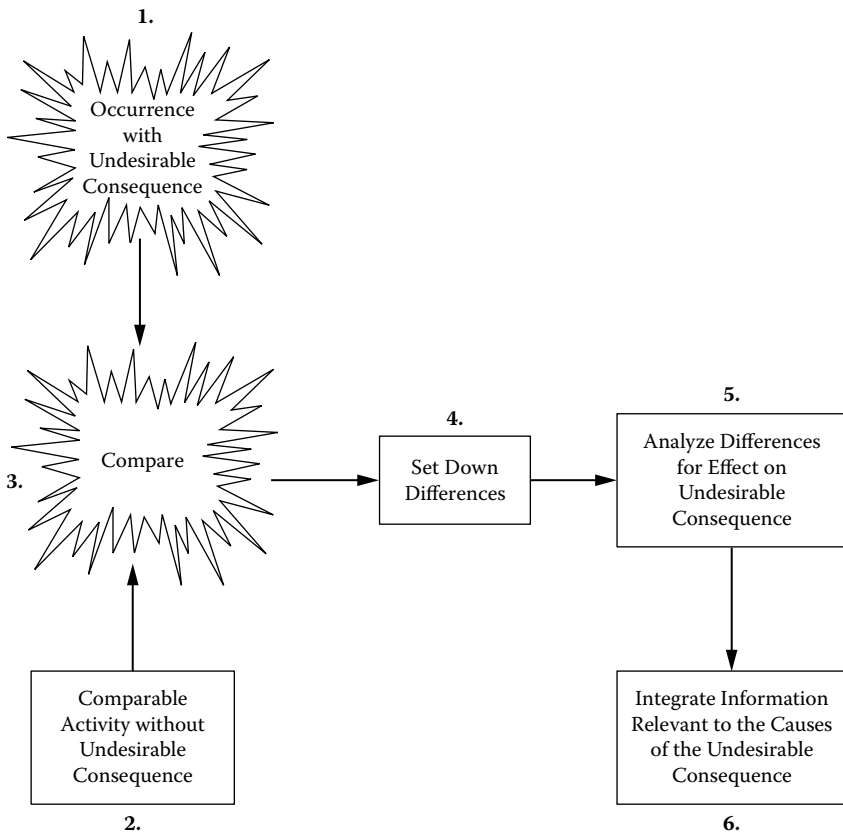
FIGURE 10.1 Six steps involved in change analysis. (Source: Courtesy of the United States Department of Energy.)
