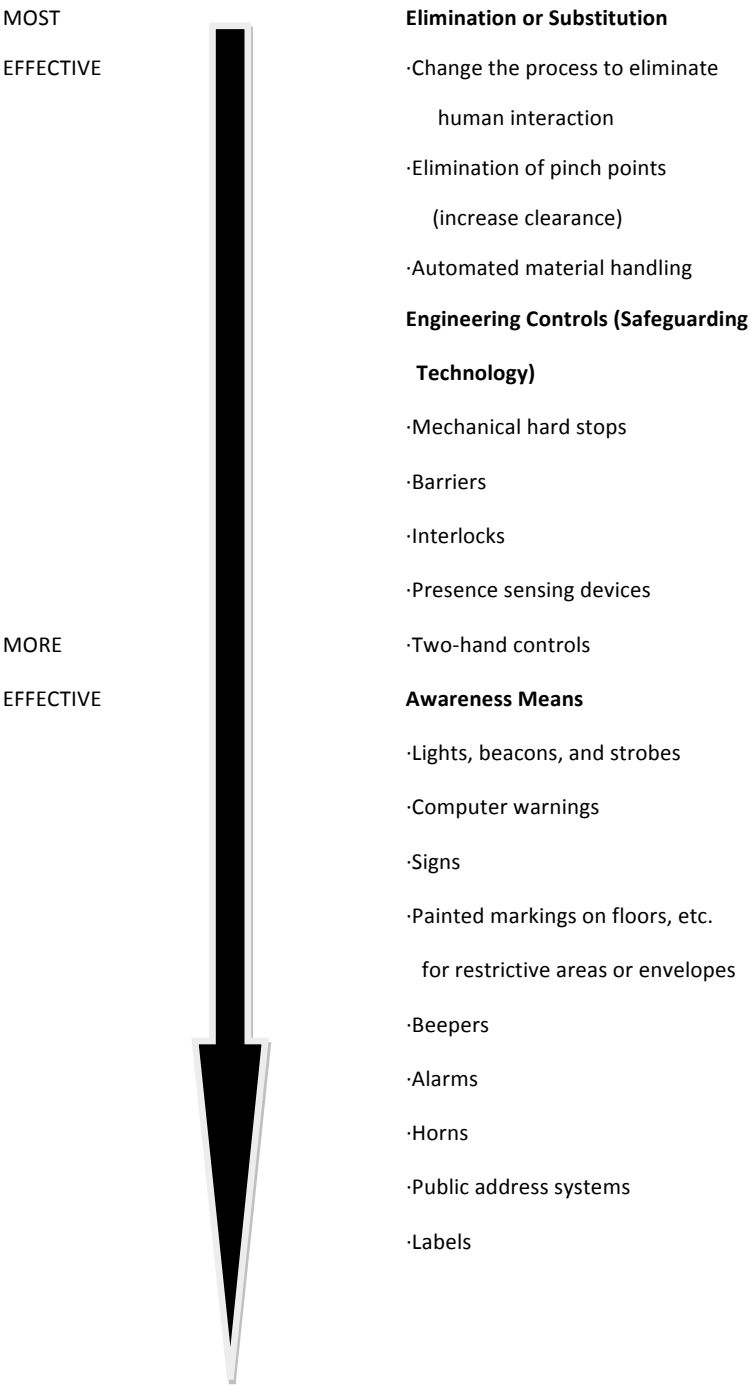
FIGURE 1.3 Ranking the effectiveness of hazard controls.
