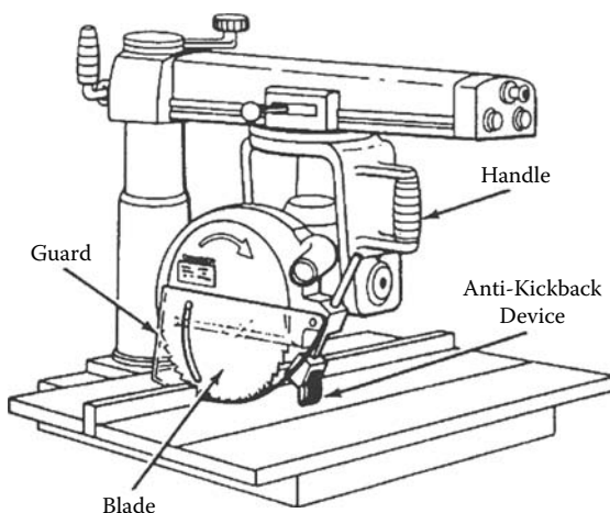
FIGURE 25.19 A self-adjusting guard for the blade of a radial saw.
