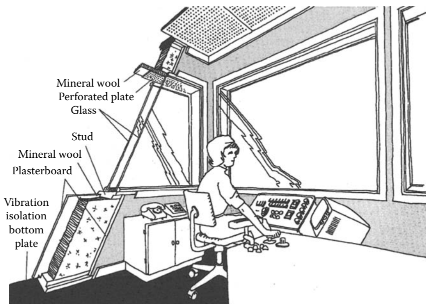
FIGURE 24.1 Typical isolation booth for a machine or equipment operator. (Courtesy of the Occupational Safety and Health Administration.)
