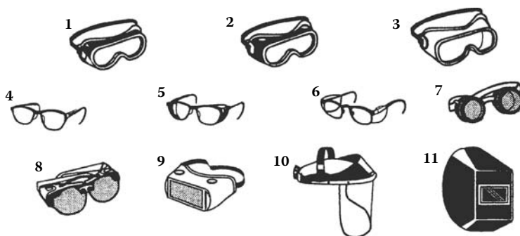
FIGURE 24.4 Types of protective eyewear. (Courtesy of the United States Department of Energy.)
