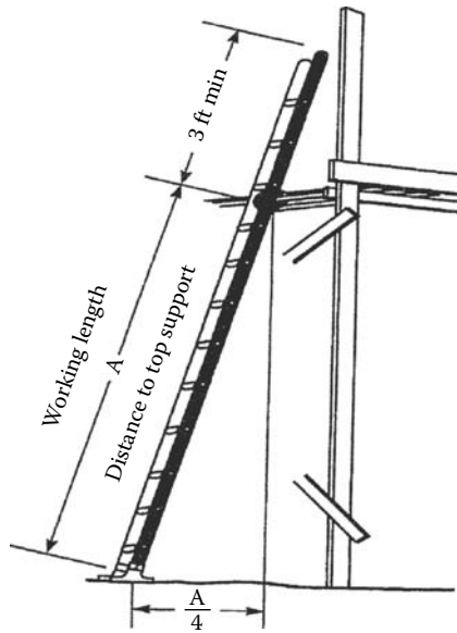
FIGURE 25.18 Safe use of portable ladder. (Source: Courtesy of the Occupational Safety and Health Administration.)
