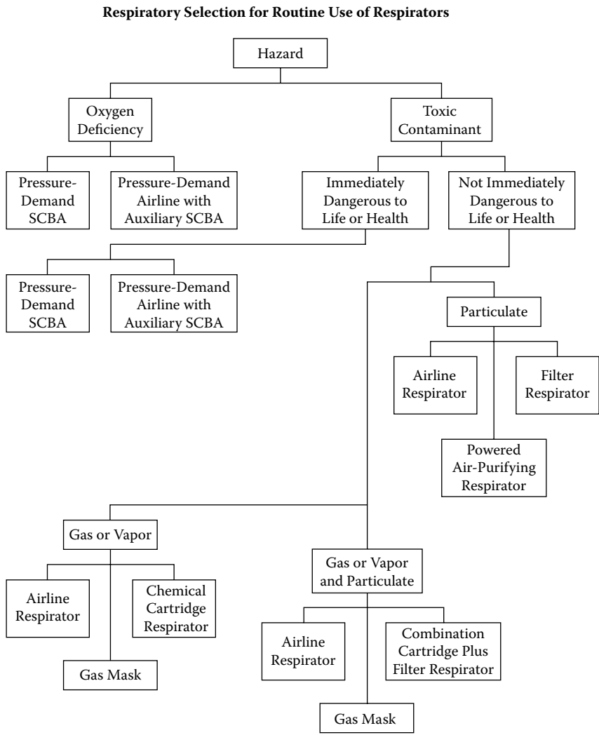
FIGURE 24.11 Respirator selection flow chart. (Courtesy of the Occupational Safety and Health Administration.)
