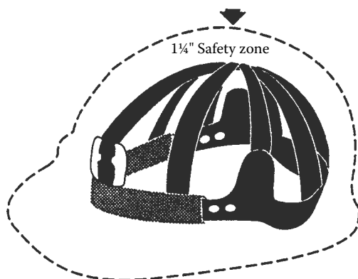
FIGURE 24.5 Head protection suspension clearance. (Courtesy of the United States Department of Energy.)
